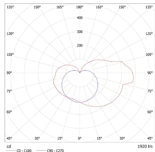
Lucis S5.L11.A450.0W ASTERION LED / LDC (Polar)
